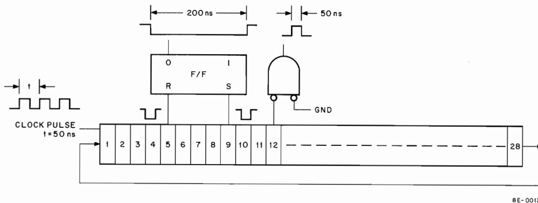
Figure 3-20 Simplified Timing Shift Register Operation
