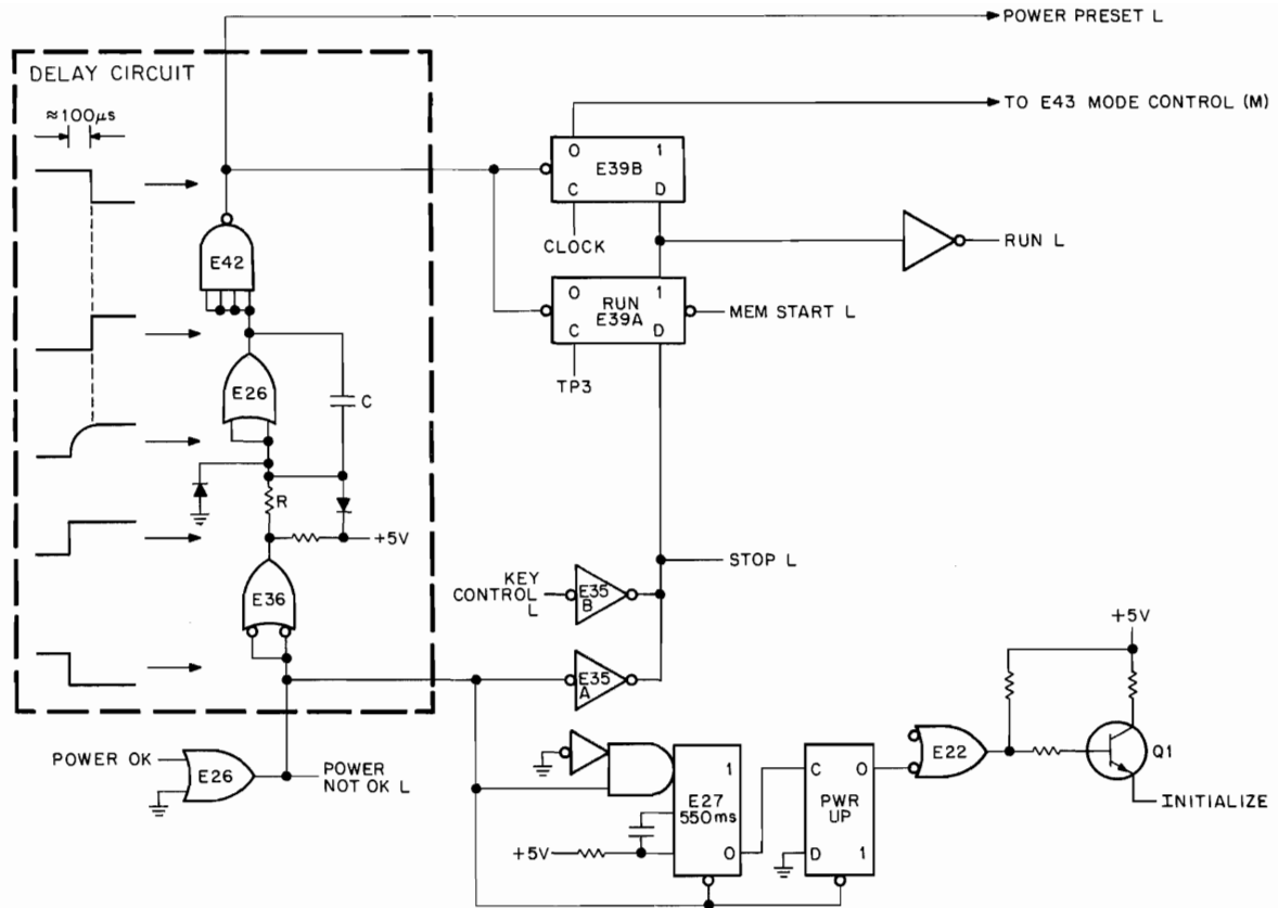
Figure 3-24 Power-On Preset Control Logic
